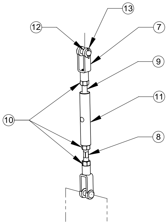
DETAIL A SCALE 1 : 6
